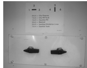
Fig. A -Water Valve Controls
