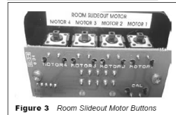
Figure 3 Room Slideout Motor Buttons
