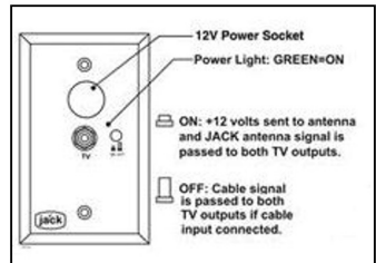
Power Injector
